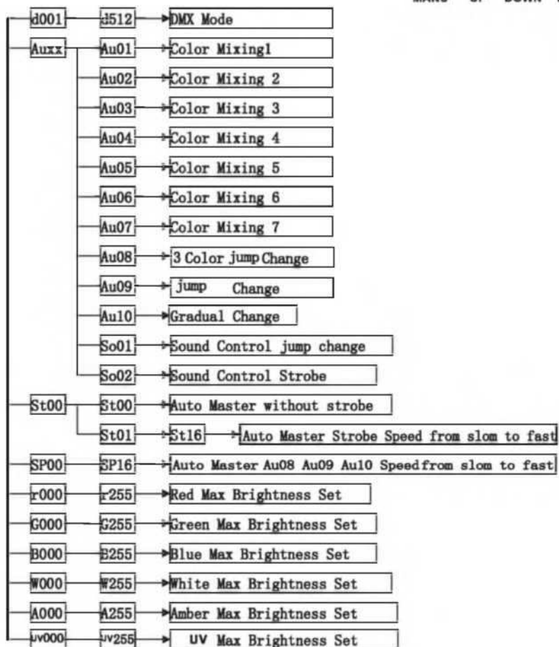
DMX5121 Control 1
